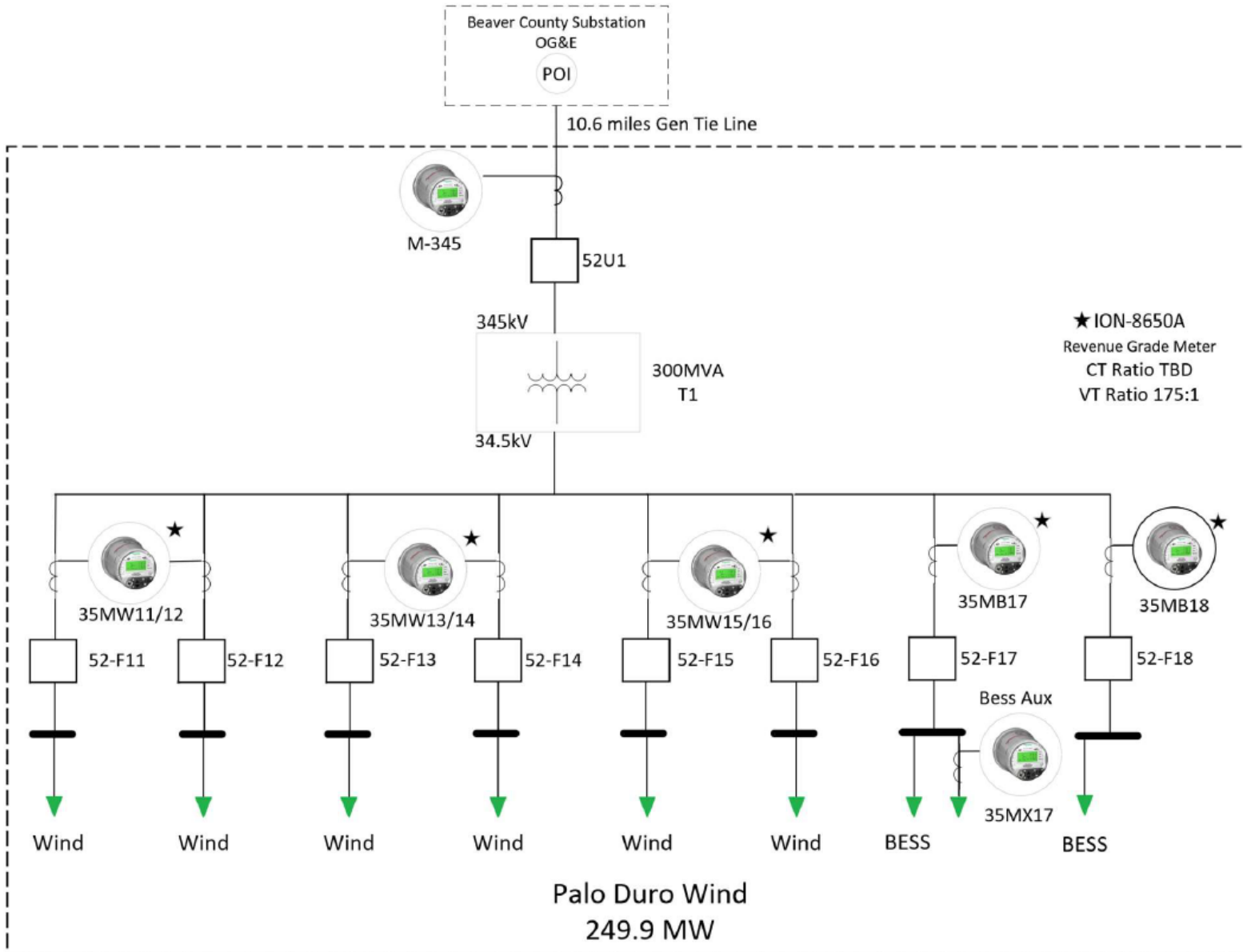
Figure 1- Simplified Metering One Line Diagram
